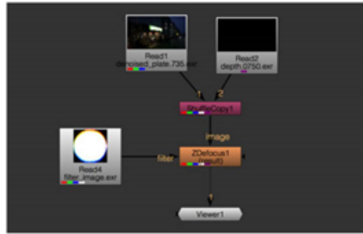
A ZDefocus script.
