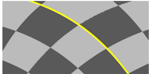
Reduced artifacts using ppass_map
