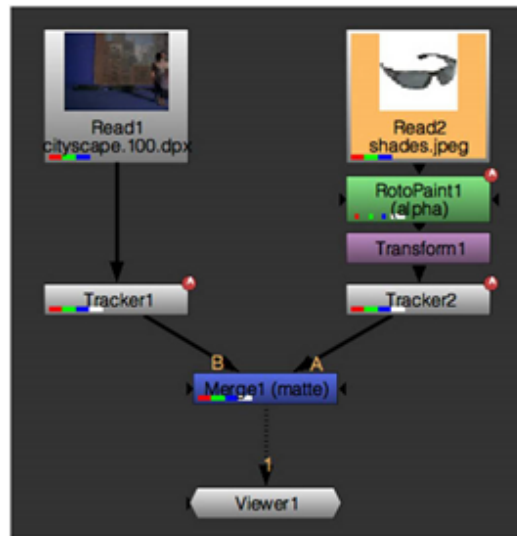
A simple match-move script.
