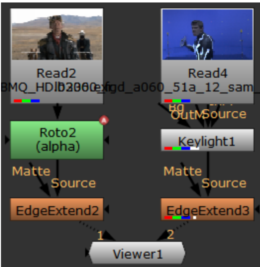
Source or keyed alpha.
