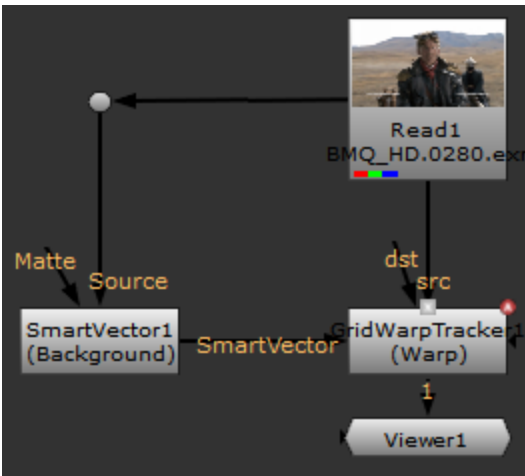
Calculating vectors in context.
