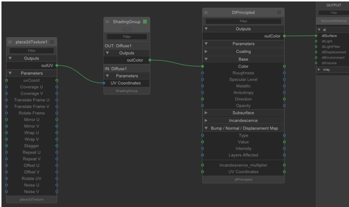
Connecting the ShadingGroup node to the rest of the Network
