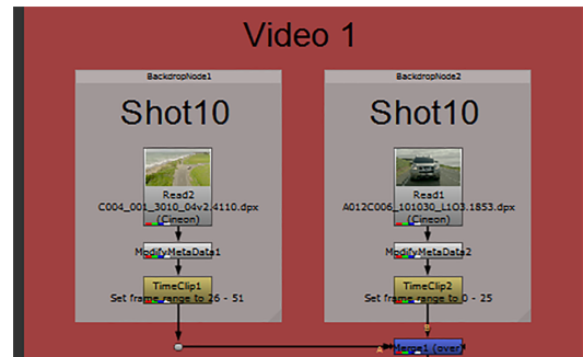
Compositing environment
