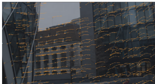
Figure 3.4: Tracking 300 features.
